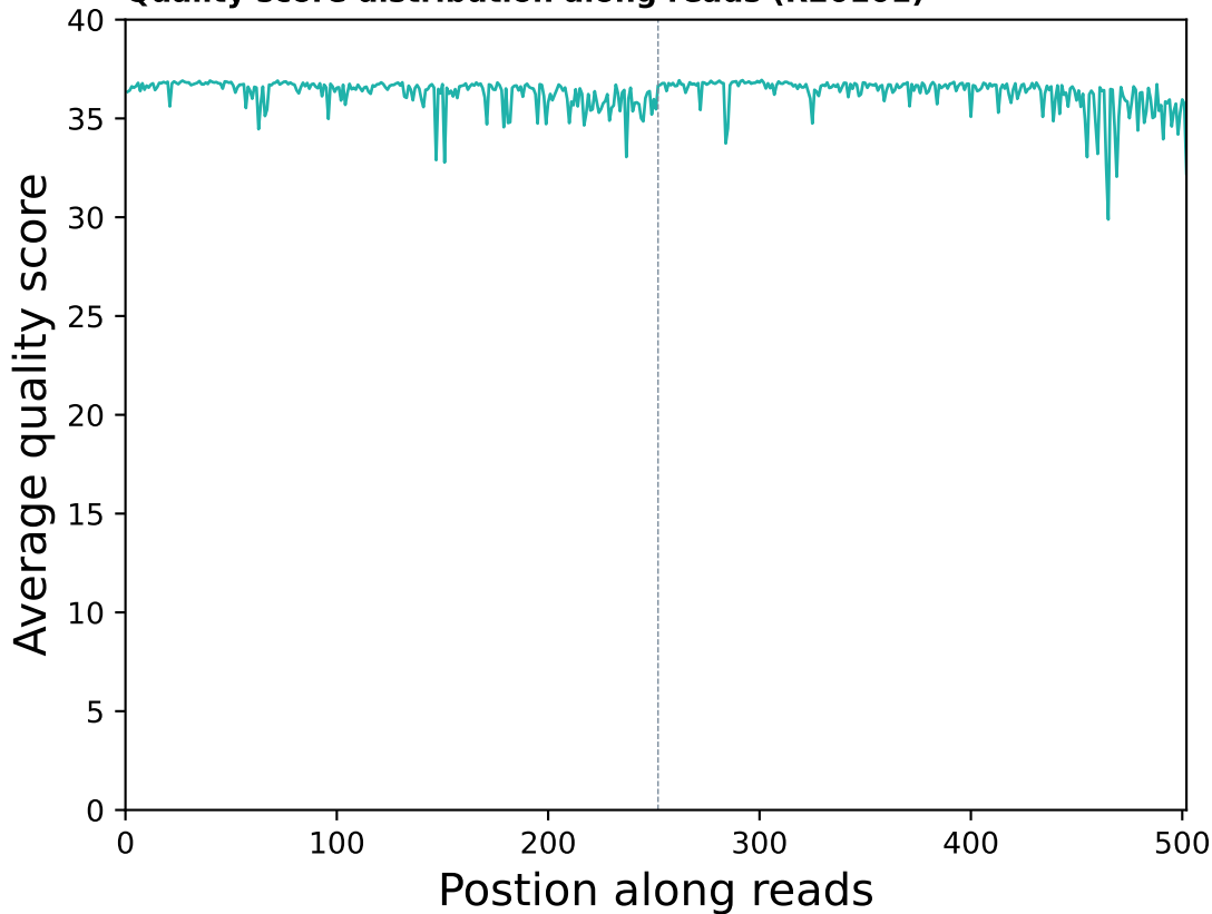
Quality score distribution along reads (R20101)
